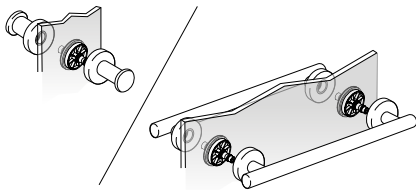
GLASS SHOWER ENCLOSURE HOLDER FOR HOOK / HOOK SOPORTE MAMPARA PARA COLGADOR / COLGADOR GLASS 6/8MM / VIDRIO 6/8MM WJC235A0042000
