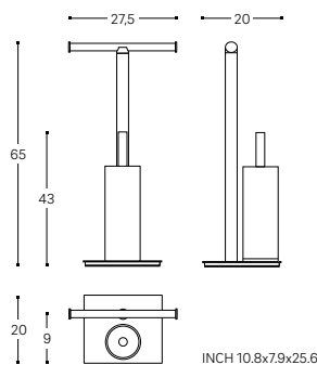
⊙○△ FREE STANDING TOILET BRUSH/PAPER HOLDER ESCOBILLERO/PORTAPAPEL SUELO
